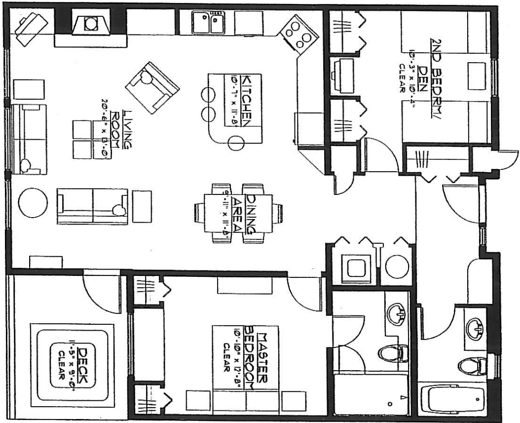
UNIT-M TWO BEDROOM (1162 sq. ft.) SCALE: NT9
